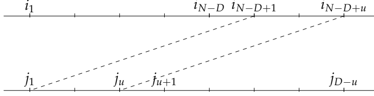
Figure 3: Pairing of indices in the concatenated code
