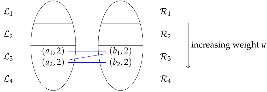
Figure 5: Edge structure of the bipartite graph in Lemma 7.8.
